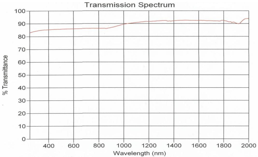
Typical Transmission 2mm thick
